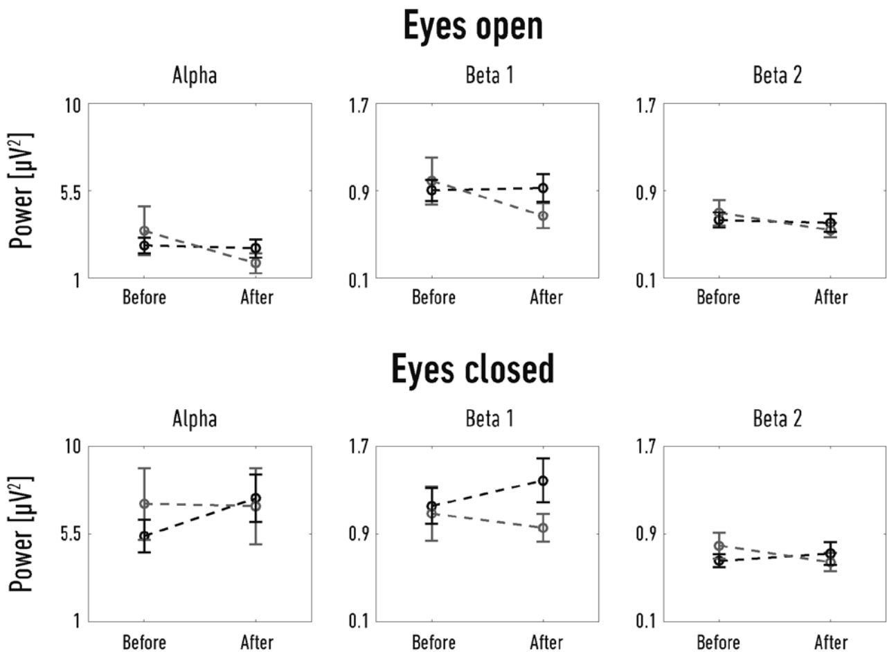
Fig. 2. Power of alpha (7.5–13 Hz), beta1 (13–20 Hz) and beta2 (20–30 Hz) bands averaged over all electrodes, for the training (black, n=14 ) and control (grey, n=10 ) groups before and after NFB training. Top row represents results for the rest with eyes open, bottom row – results for the rest with eyes closed. Error bars represent standard error of the mean.
